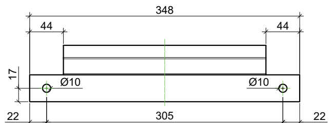
BRACKET DETAIL TOP VIEW
